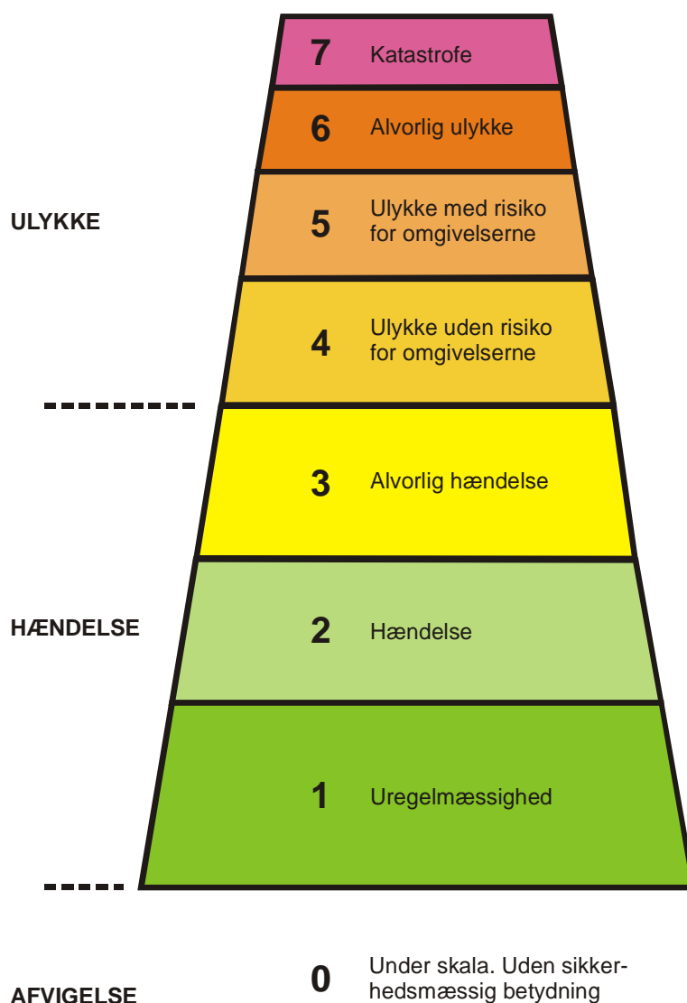
Figur 1 INES skalaen
